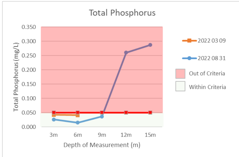
Figure 8: Total phosphorus from Kemmerer samples of Elinor Lake – 2022
