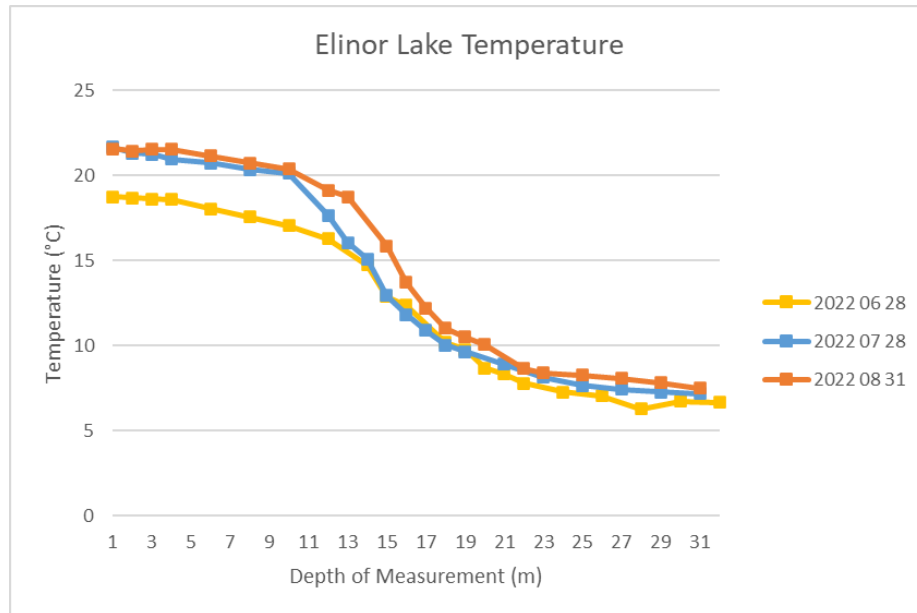
Figure 4: Elinor Lake temporal and spatial temperature measurements – 2022
