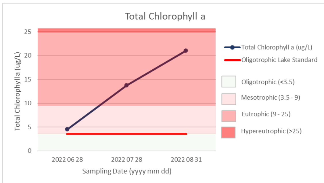
Figure 9: Total Chlorophyll-a from Composite samples of Elinor Lake – 2022
