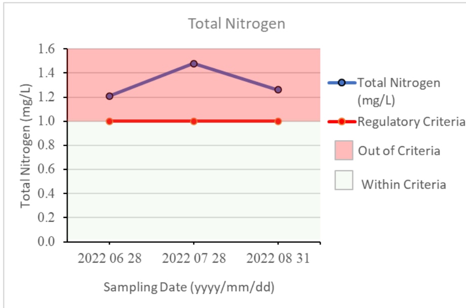
Figure 5: Total nitrogen from composite samples of Elinor Lake – 2022
