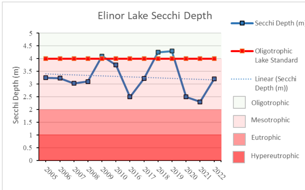
Figure 10: Historical trend for Secchi Depth in Elinor Lake
