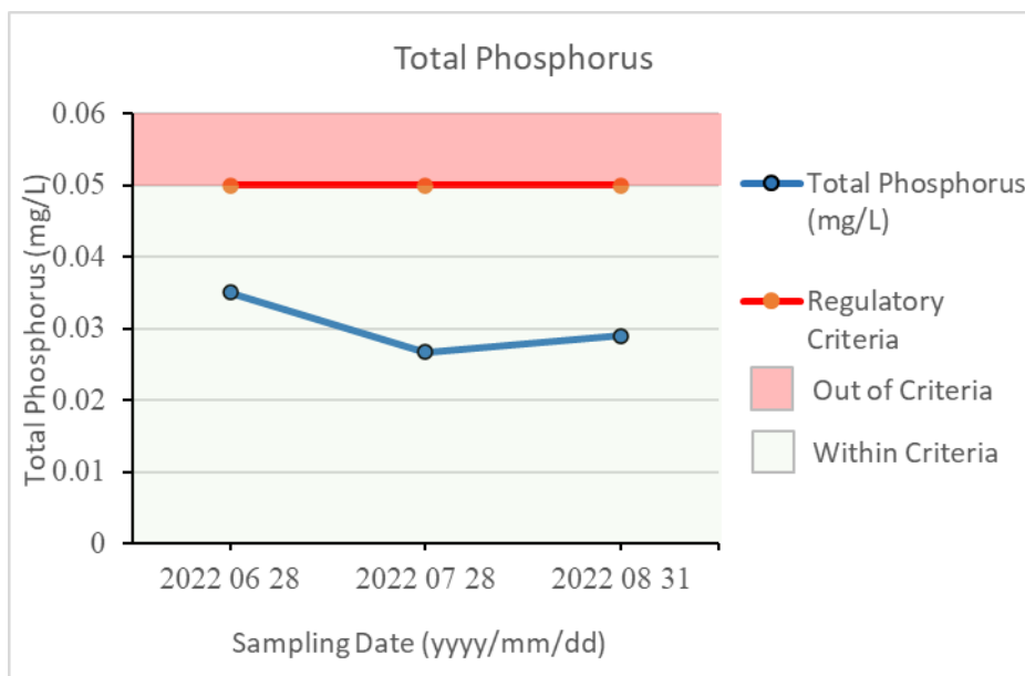
Figure 7: Total phosphorus from composite samples of Elinor Lake - 2022
