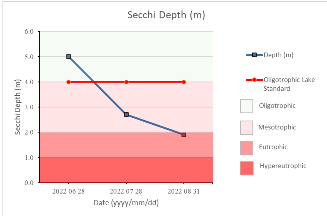
Figure 2: Secchi depth measurements in Elinor Lake - 2022
