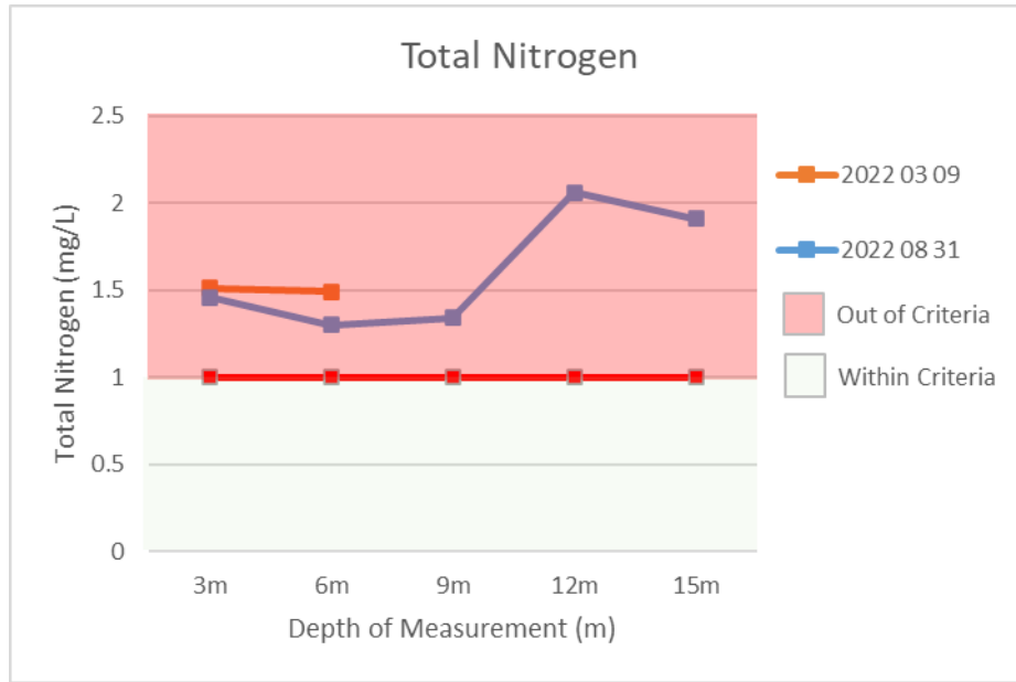
Figure 6: Total nitrogen from Kemmerer samples of Elinor Lake – 2022
