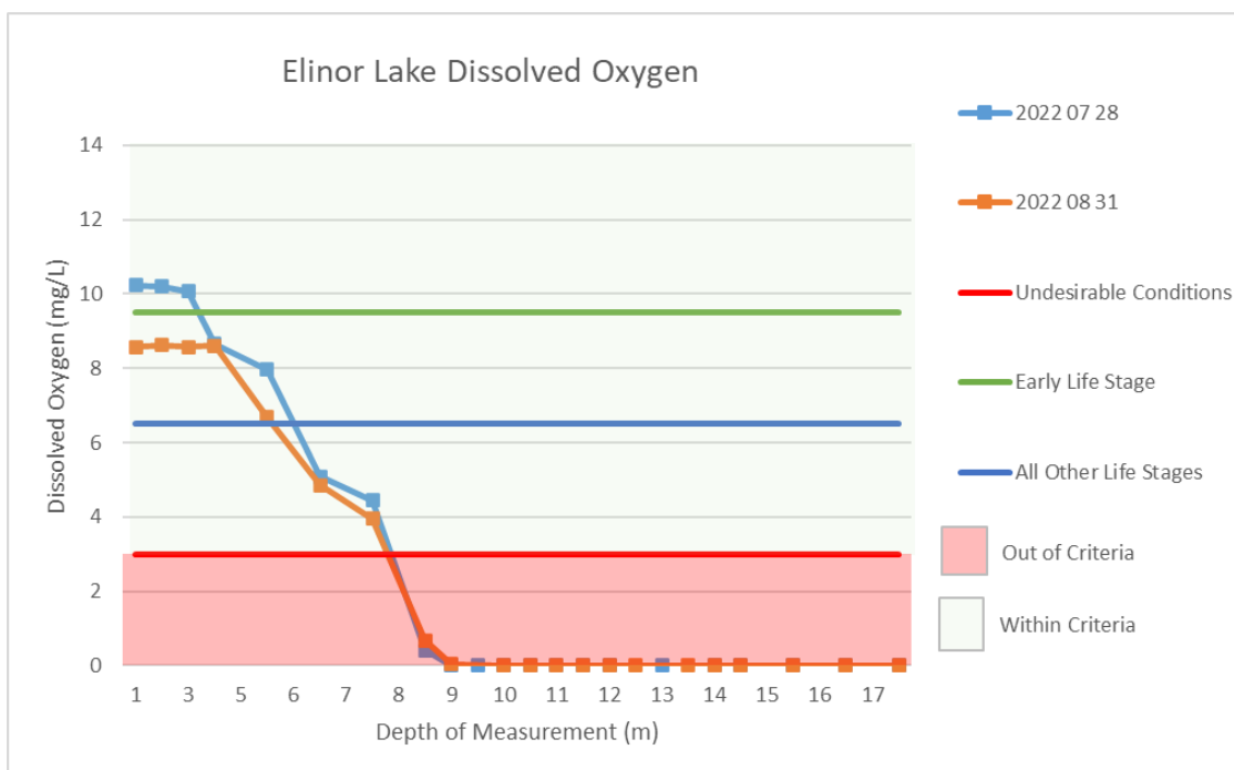
Figure 3: Dissolved oxygen in in Elinor Lake – 2022
