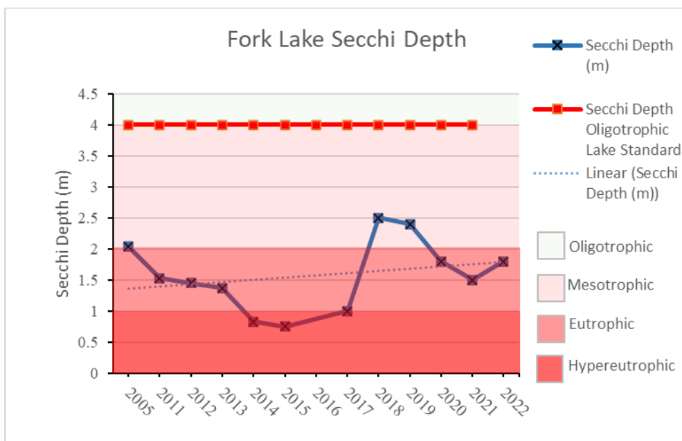
Figure 10: Historical trend for Secchi Depth in Fork Lake
