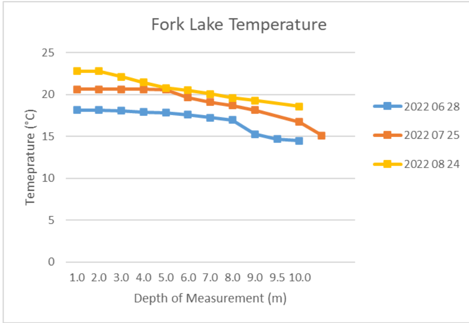
Figure 4: Temperature profile in Fork Lake – 2022
