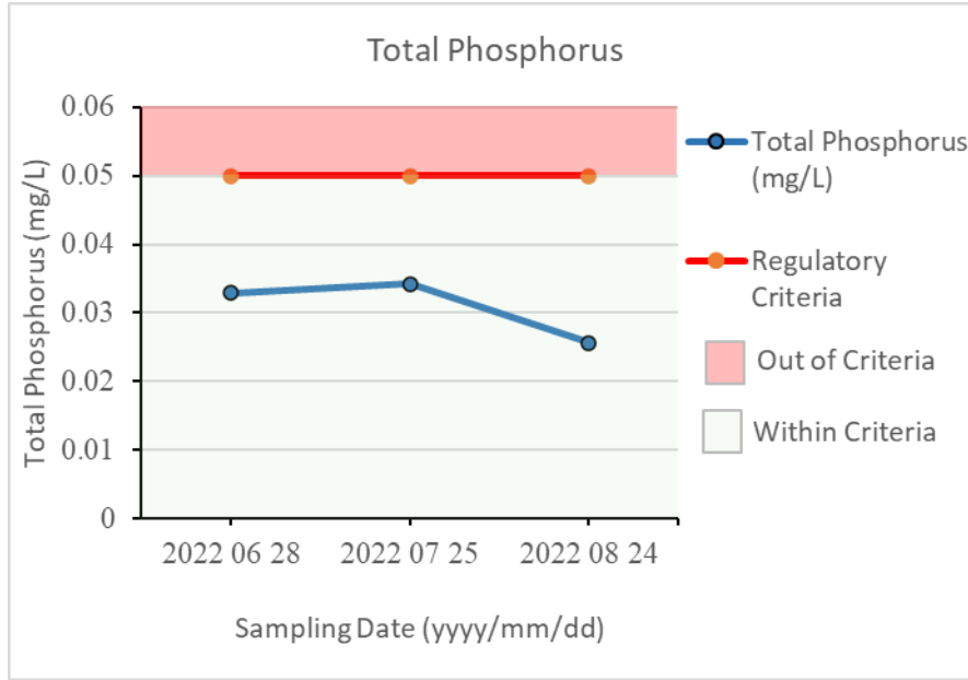
Figure 7: Total phosphorus in composite samples of Fork Lake - 2022
