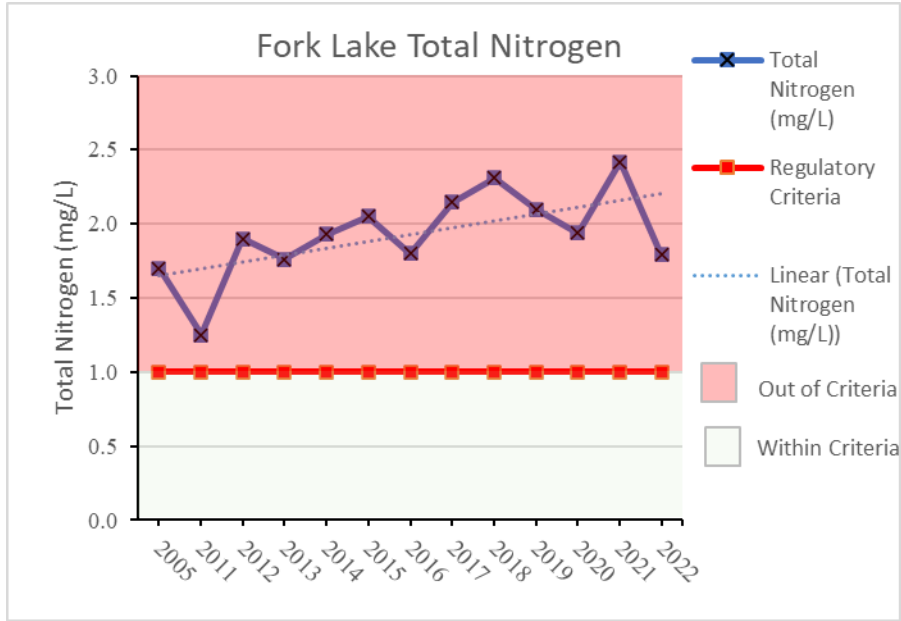
Figure 11: Historical trend of total nitrogen concentrations in in Fork Lake
