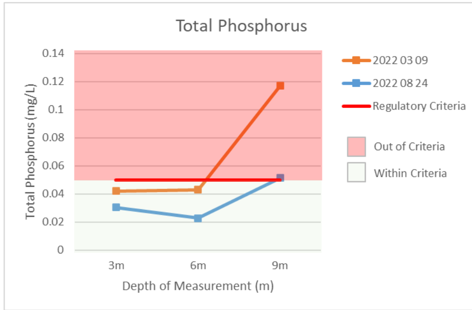
Figure 8: Total phosphorus from Kemmerer samples of Fork Lake – 2022
