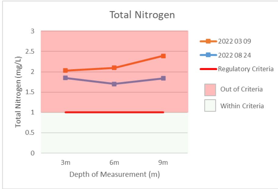
Figure 6: Total nitrogen from Kemmerer samples of Fork Lake - 2022
