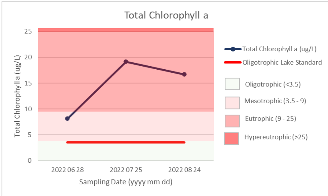
Figure 9: Total Chlorophyll-a in Composite samples of Fork Lake - 2022
