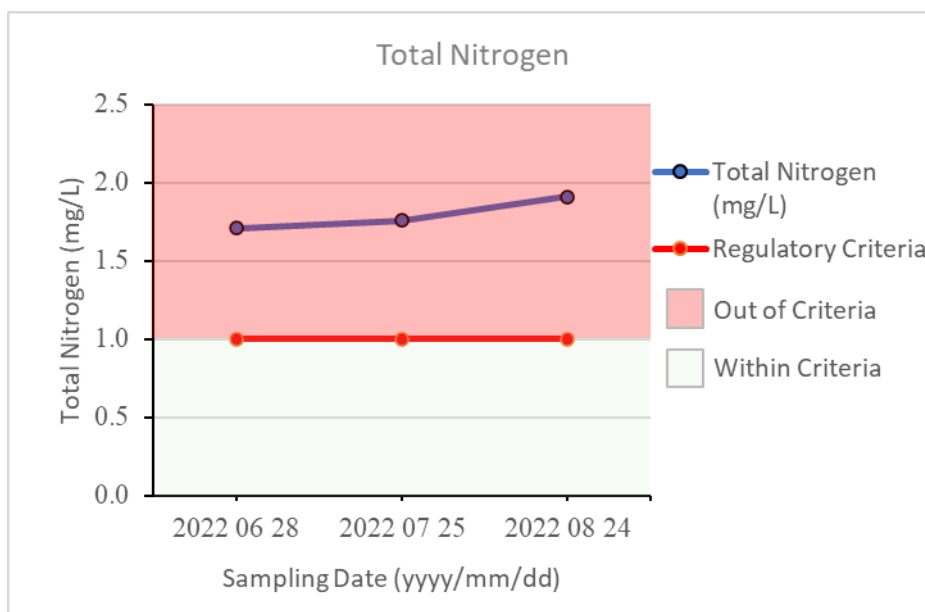
Figure 5: Total nitrogen from composite samples of Fork Lake – 2022
