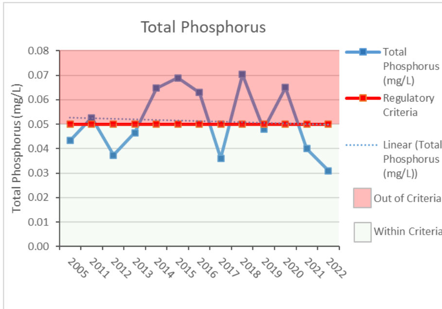
Figure 12: Historical trend of total phosphorus concentrations in Fork Lake
