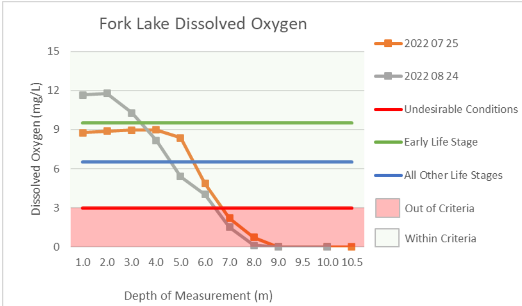
Figure 3: Dissolved oxygen in Fork Lake – 2022
