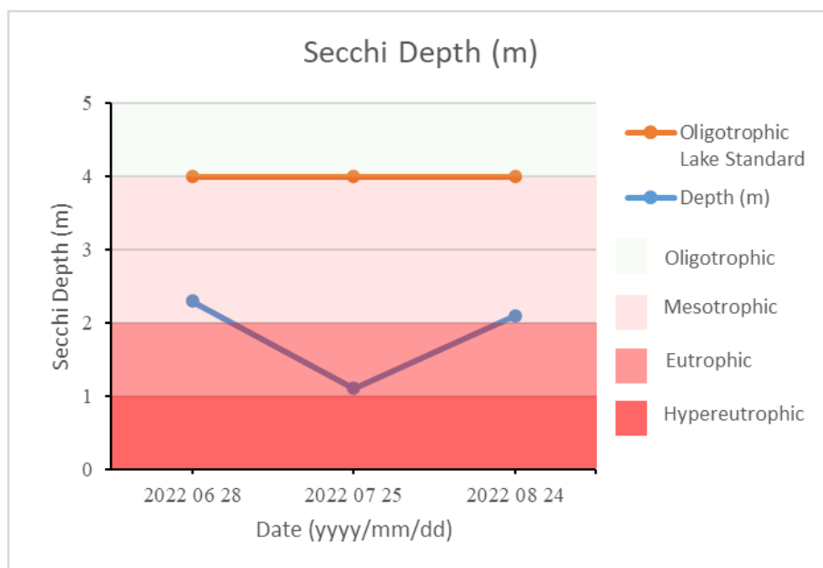
Figure 2: Secchi depths measured in Fork Lake – 2022
